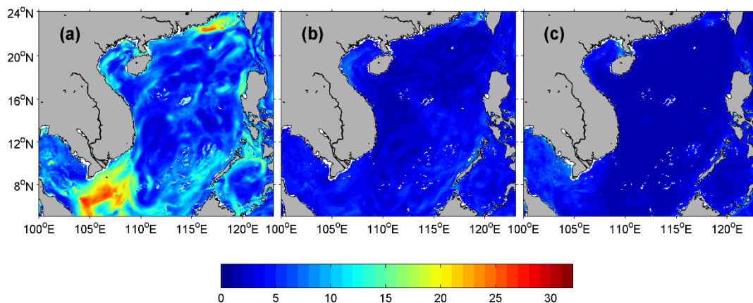
Figure 2 Maps of the S/N ratio for (a) the first box EOF 1-10, (b) the second box EOF 11-50, (c) the third box EOF 51-1400.
