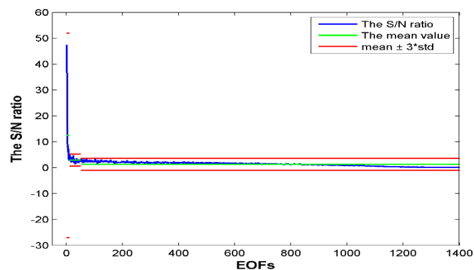
Figure 1 The S/N ratios as a function of EOF index. Small scales are situated at the right end, large-scales at the left end. Based on the distribution of the S/N ratio, the scales (EOFs) are divided into three boxes, EOF 1-10, EOF 11-50 and EOF 51-1400. The green line in each box is the mean value of the ratio values, and the red lines above and below the green line in each box are the mean value \pm 3 standard deviation of the S/N ratio in the same box, respectively.
