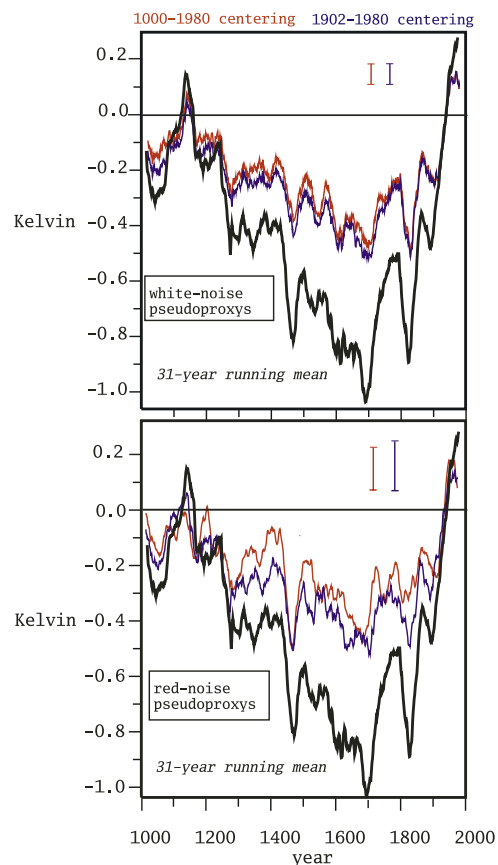
Figure 1. Time-filtered Northern Hemisphere annual near-surface air temperature anomalies in the last millennium (relative to the mean of the calibration period 1902–1980), as simulated with the model ECHO-G [ von Storch et al., 2004 ] (black thick line), and resulting from the application of the MBH98 algorithm to a network of pseudo-proxies taken from the same simulation and degraded with stochastic noise (thick colored lines: one noise realization close to the mean of 100 realizations). The variance of the pseudoproxies contains 50% reconstruction scatter (after time filtering) estimated from 100 realizations of the noise. The reconstruction with 1900–1980 centering is given in red, the one with full centering in blue.
