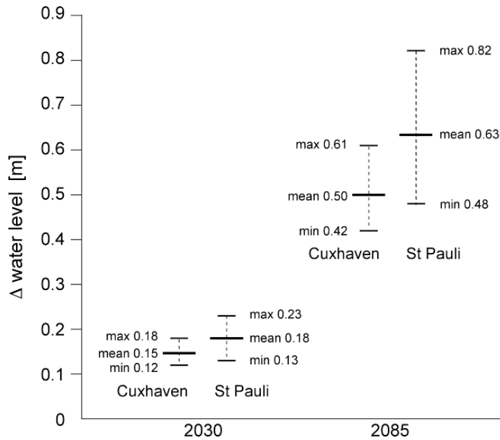
Fig 6: Scenarios of changes in extreme high waters (incl. sea level rise) in Cuxhaven and St. Pauli, 2030 and 2085, based on TRIMGEO simulations forced with winds and air pressure from different regional models and emissions scenarios. Since the A2 and B2 scenarios do not differ significantly we indicate the mean value across all models and scenarios and the minimum maximum range
