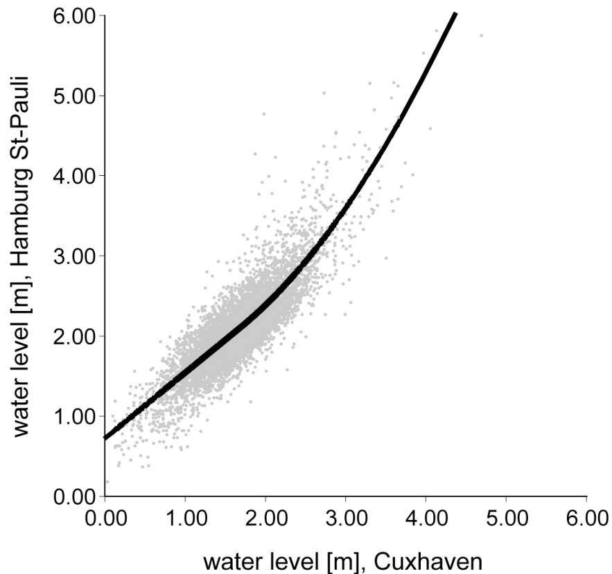
Fig.4: Linear–quadratic fit for the observed high water levels at Hamburg St. Pauli (vertical axis) and those modeled for the coastal grid box 53.8°N / 8.8°E (Cuxhaven; horizontal axis). Units: m
