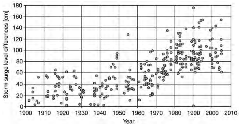
Fig. 2: Differences between extreme high waters in St. Pauli and Cuxhaven (in cm). Due to dredging of the waterway and coastal defense measures the difference has grown during the 1960s and 70s, but since about 1980 conditions are stationary. Courtesy of Hamburg Port Authority, Hydrology
